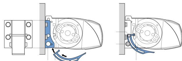
Fig. 2.3 Detail middensteun B
