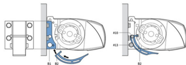
fig. 2.3 Detail middensteun B
